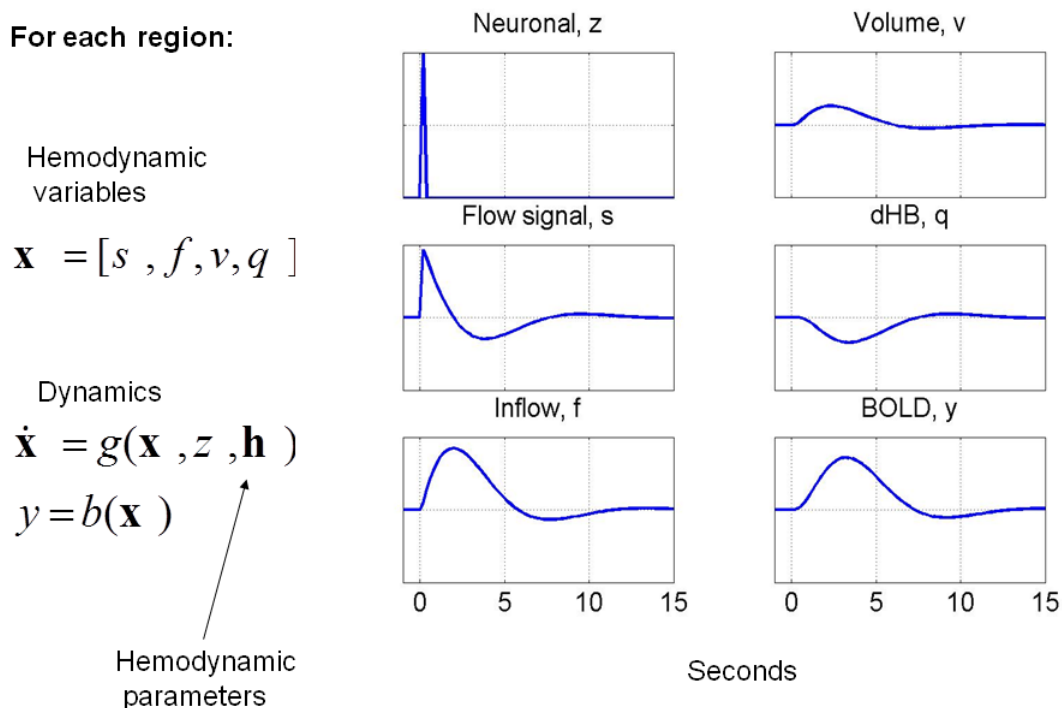
Figure 1.7: Hemodynamics generated using the extended Balloon model [Friston, 2002b] in response to a brief stimulus. These signals correspond to the equations plotted in Figure 1.6. A more detailed description of the model and parameters is presented in Chapters 5 and 6.
